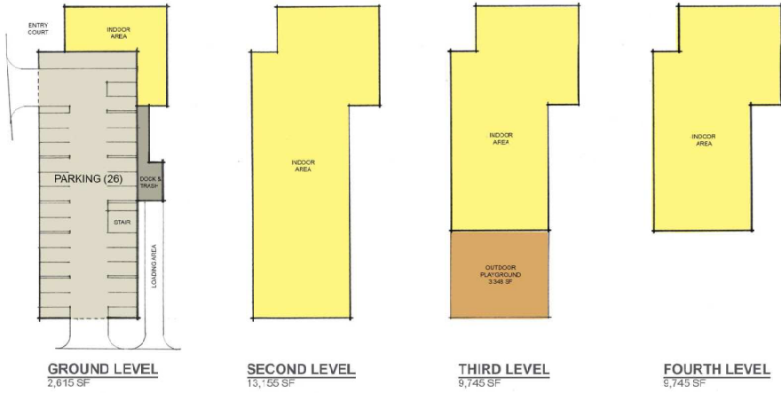
BUILDING DIAGRAMS Scale: 1" = 30'-0"
